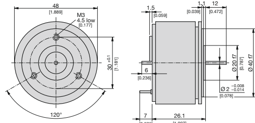
Fig. 2. KINAX 2W2 with special drive shaft at front and at rear. At front: dia. 2 mm, length 12 mm [0.078", 0.472"]. At rear: dia. 2 mm, length 6 mm [0.078", 0.236"]
