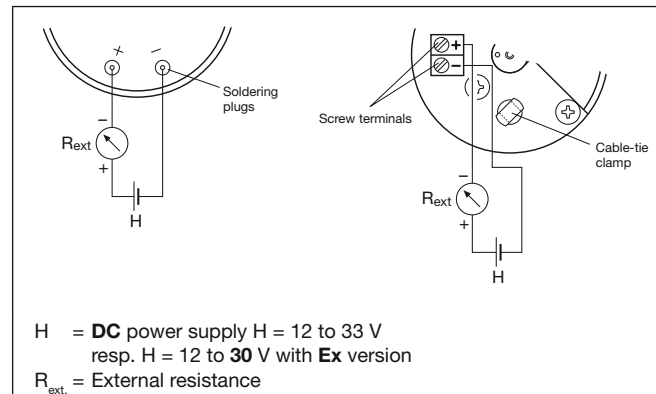
Fig. 10. Connection diagrams for 2-wire connection.
