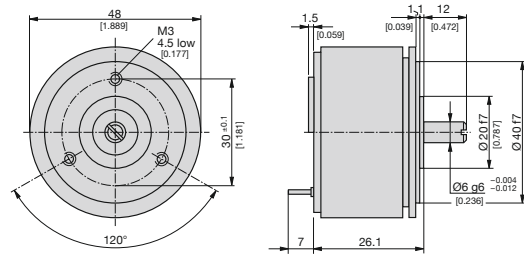
Fig. 3. KINAX 2W2 with special drive shaft at front only , dia. 6 mm, length 12 mm [0.236", 0.472"]
