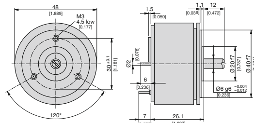
Fig. 4. KINAX 2W2 with special drive shaft at front and at rear. At front: dia. 6 mm, length 12 mm [0.236", 0.472"]. At rear: dia. 2 mm, length 6 mm [0.078", 0.236"]
