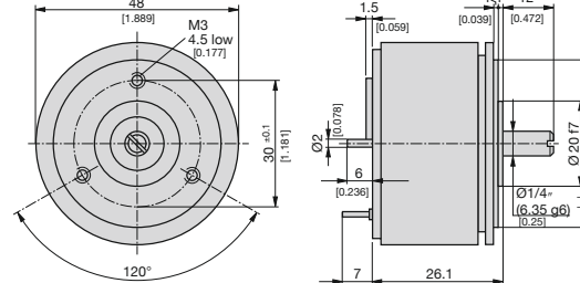
Fig. 6. KINAX 2W2 with special drive shaft at front and at rear. At front: dia. 1/4", length 12 mm [0.472"]. At rear: dia. 2 mm, length 6 mm [0.078", 0.236"]
