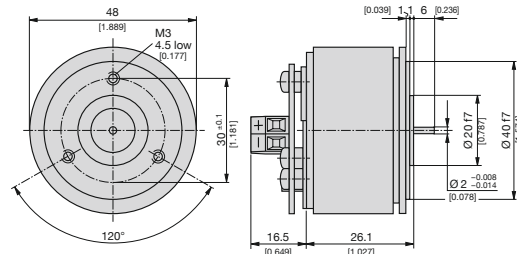
Fig. 1. KINAX 2W2 with standard drive shaft at front only , dia. 2 mm, length 6 mm [0.078", 0.236"], screw terminal version.
