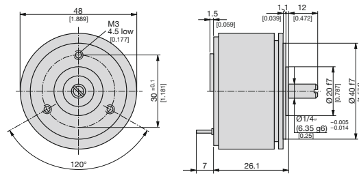
Fig. 5. KINAX 2W2 with special drive shaft at front only , dia. 1/4", length 12 mm [0.472"]
