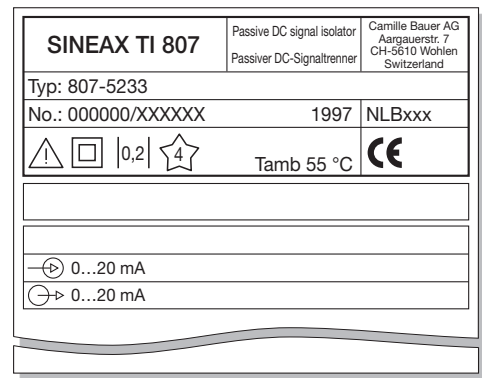
Fig. 7. Example of a nameplate.
