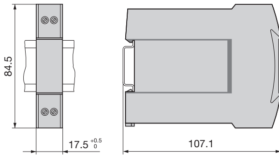
Fig. 12. SINEAX TI 807-5.... (housing N17) clipped onto a top-hat rail (35 x 7.5 or 35 x 15 mm, acc. to EN 50022).
